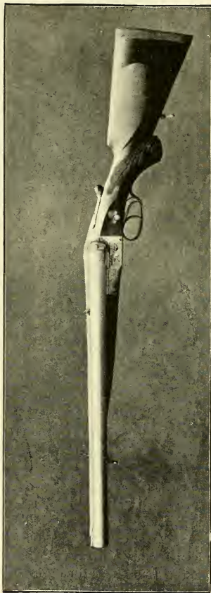
Hammerless 8-calibre 13 lb. Elephant Rifle, with 22-inch Barrels and full Pistol Hand and Check-piece to Stick.
